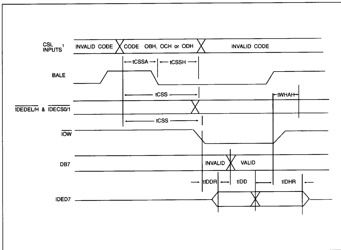
FIGURE 10-18. IDE INTERFACE W/BALE TIMING (DB7 to IDED7)
