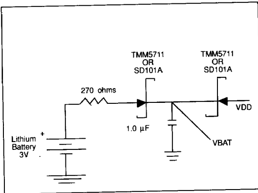
FIGURE 7-2. VBAT EXTERNAL SUPPORT
