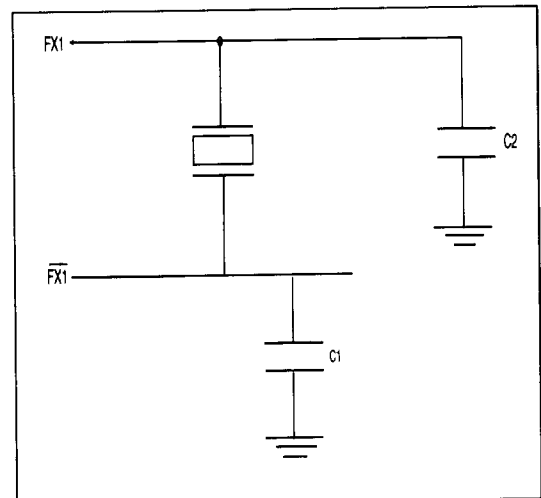
FIGURE 5-1. 16 MHZ CRYSTAL
