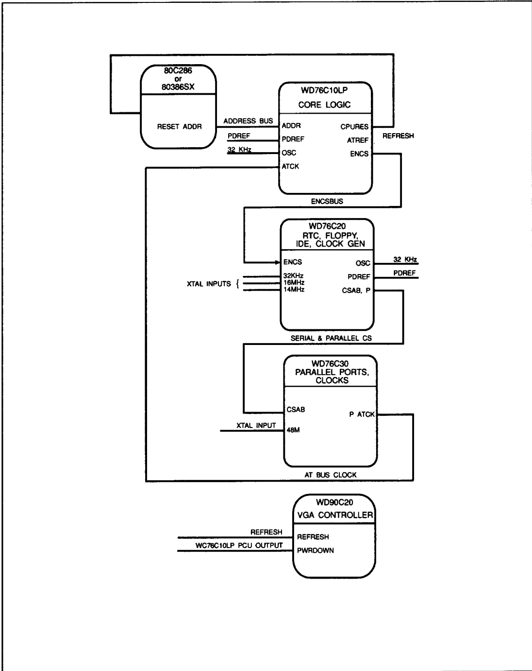
FIGURE 8-2. FULL POWER-DOWN MODE SYSTEM BLOCK DIAGRAM
