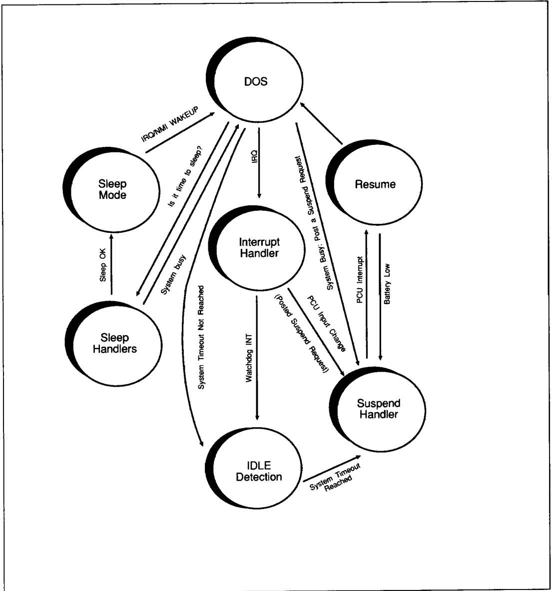
FIGURE 8-1. SUSPEND/RESUME/SLEEP MODE CYCLE
