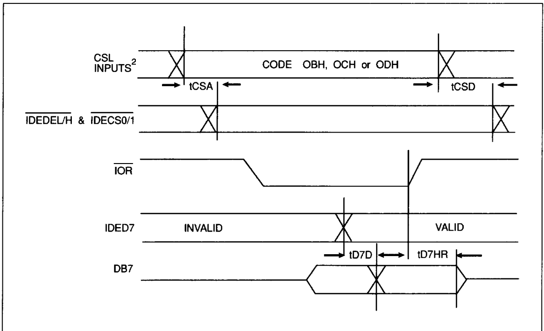
FIGURE 10-15. IDE INTERFACE TIMING DIAGRAM ( \overline{\text{IDED7}} TO DB7)
