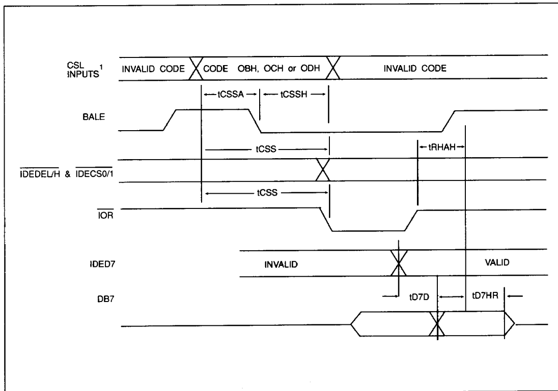
FIGURE 10-16. IDE INTERFACE W/BALE TIMING (IDED7 to DB7)
