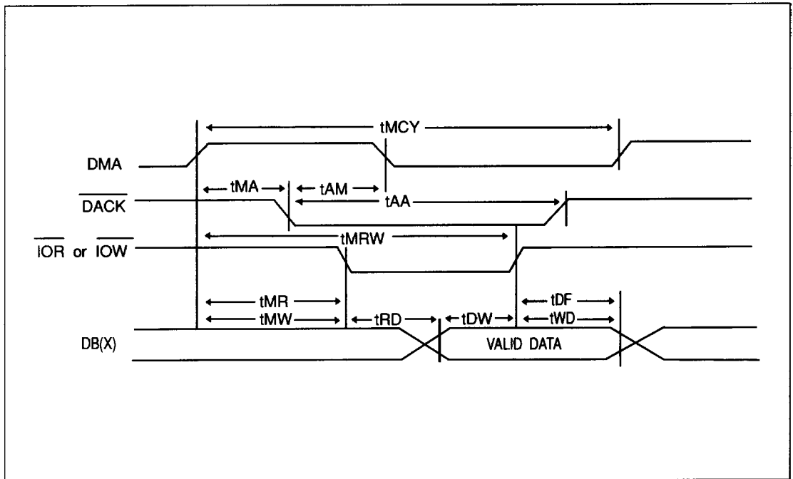
FIGURE 10-5. FDC DMA TIMING DIAGRAM
