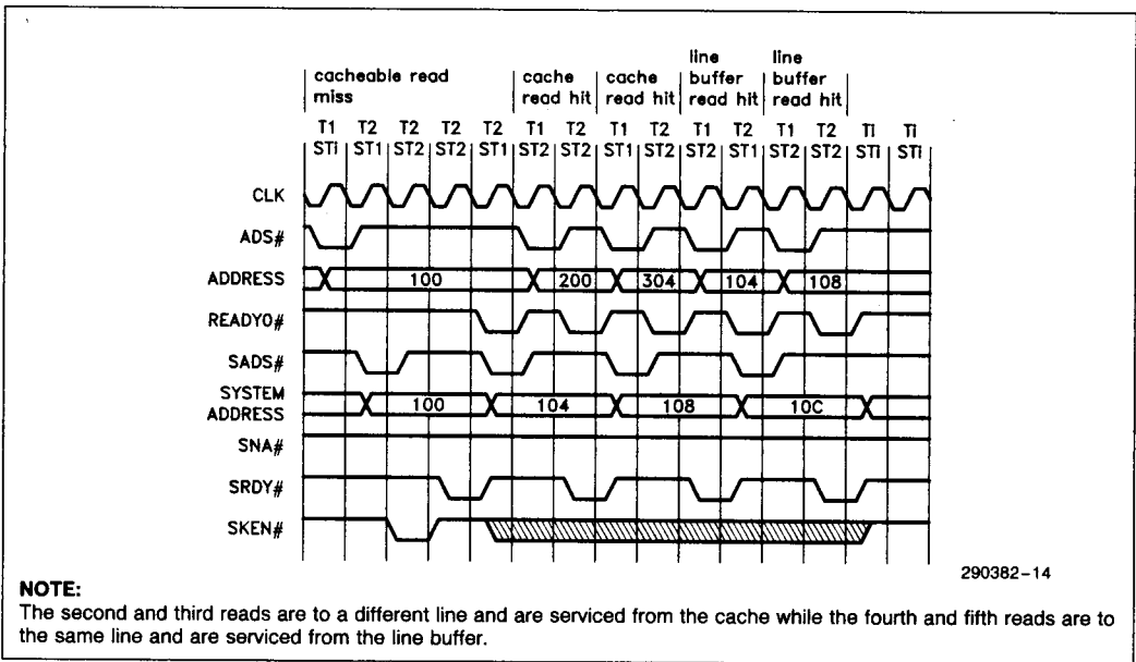
Figure 4.1 - Read Hit Cycles During a Line Fill
