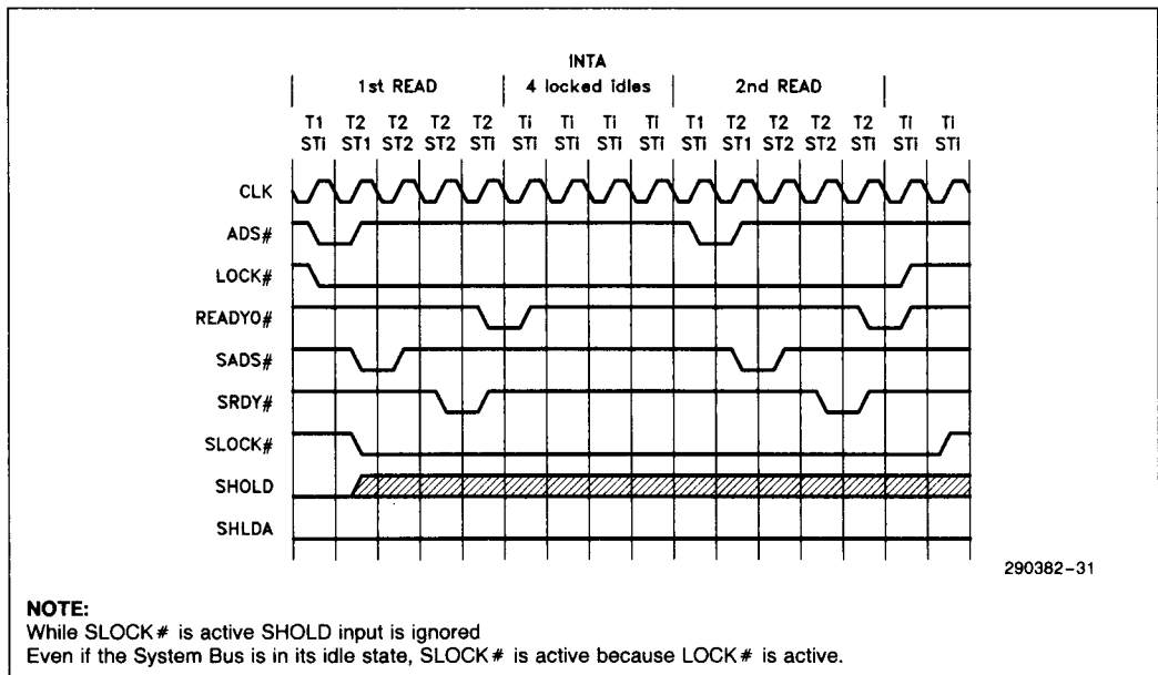
Figure 6.7 - INTA LOCK# ed Cycle
